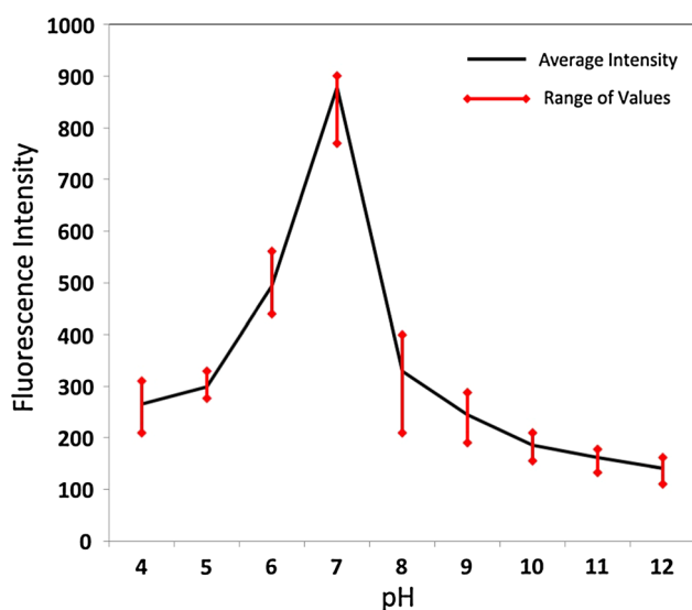
Figure 6 \text{Fe}_3\text{O}_4@\text{Pt} NCs under different pH conditions were prepared five times and their fluorescence intensity was performed.
